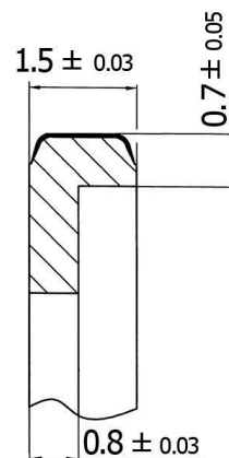
Detaliu segment piston Piston ring detail
